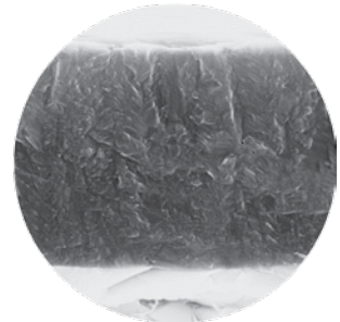
nc-ALTiN coating nc-ALTiN Beschichtung
